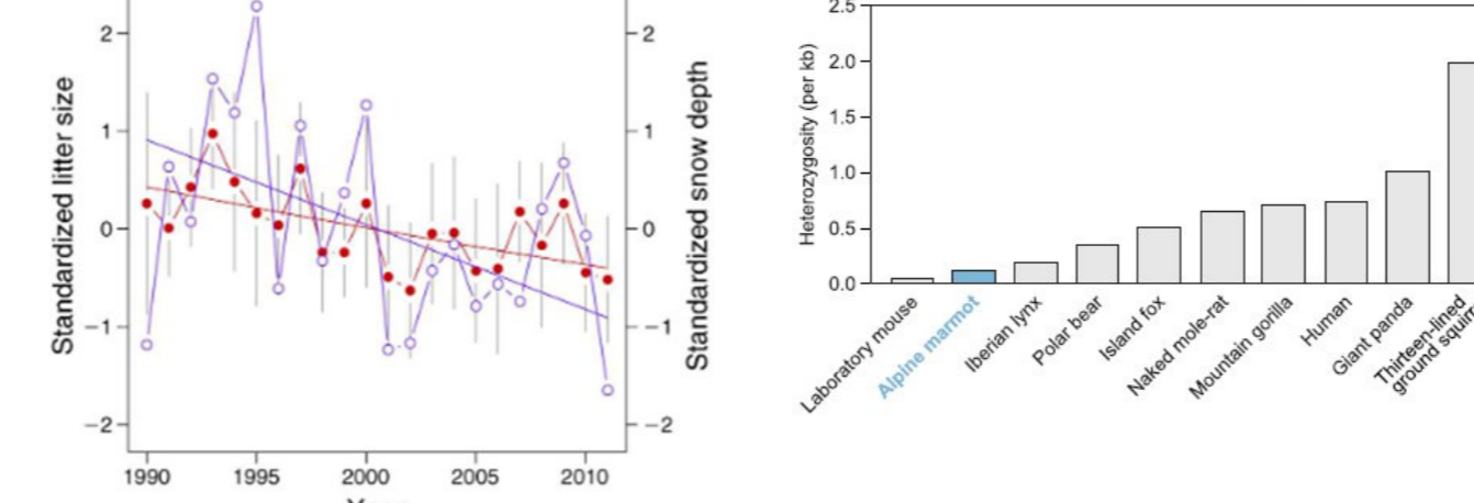
Source : Marion TAFANI, Aurélie COHAS, Christophe BONENFANT, Jean-Michel GAILLARD, et Dominique ALLAINE ? 2013. Decreasing litter size of marmots over time: a life history response to climate change? Ecology, 94(3), pp. 580-586
